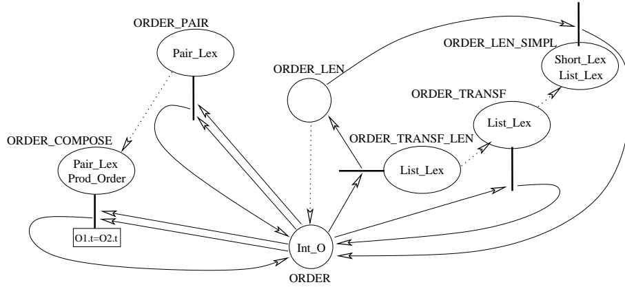
Fig. 1. A representation of the set \mathcal{A} of modules, functors, and signatures as given in the text. Each vertex corresponds to a signature: simple vertices for module signatures, and vertices with “handles” for functor signatures. Each parameter signature is linked to the handle of its functor, which is in turn linked to the result signature. Each vertex-signature contains all of the components in \mathcal{A} which satisfy it. The dotted arcs denote compatibility (subtype) relationships. The labeled handle of ORDER_COMPOSE (a constrained version of ORDER_PAIR ) indicates its involved type sharing constraint. Applying the available functors yields new components which can also take their place in the vertices.
