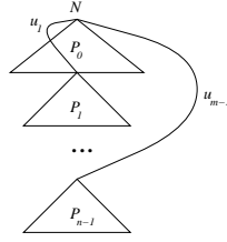
Figure 11.3: A tower of strict preredexes
