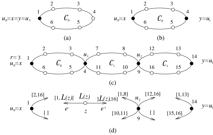
Fig. 3. Construction of the proof of Lemma 2.
