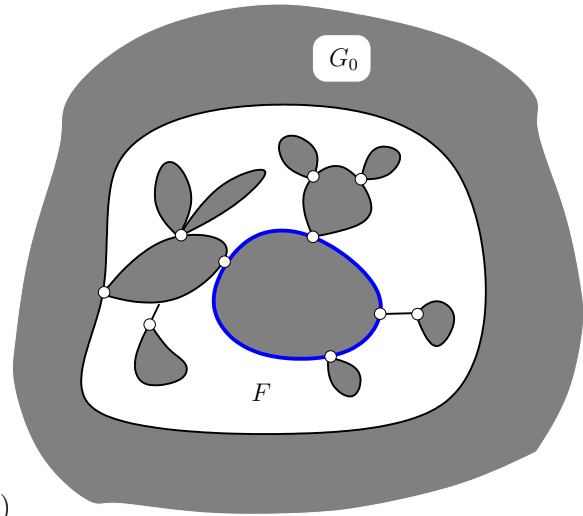
Figure 1: (a) A uniform weighted graph with 19 vertices that is not face-separable whereas all its bicomponents are. (b) Graph G_0 is depicted rayed, and face-separator B_0 , which is not biconnected, is the border of face F . The face-separator provided by Claim 1 is drawn blue. To make B the border of a face, the embedding of G_0 has to be changed.
