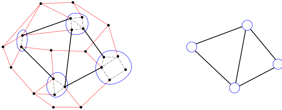
Figure 4: A graph G and a minor H .
