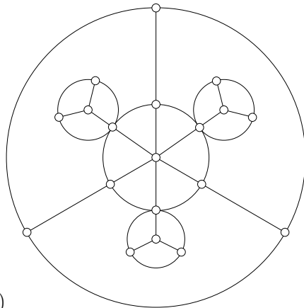
Figure 1: (a) A uniform weighted graph with 19 vertices that is not face-separable whereas all its bicomponents are. (b) Graph G_0 is depicted rayed, and face-separator B_0 , which is not biconnected, is the border of face F . The face-separator provided by Claim 1 is drawn blue. To make B the border of a face, the embedding of G_0 has to be changed.
