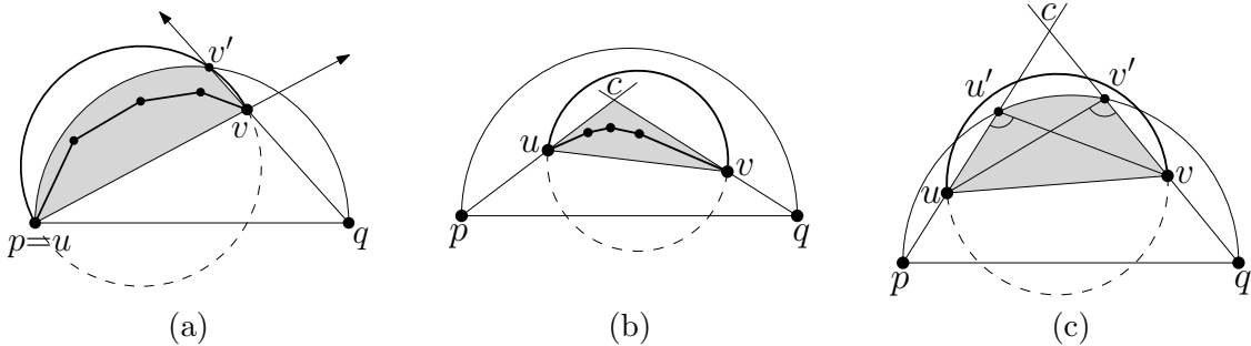
Figure 2: Proof of Theorem 6: the path \delta_C(u, v) is inside the shaded regions, where (a) u = p and v \neq q , (b) u \neq p , v \neq q , and c \in D(p, q) , and (c) u \neq p , v \neq q , and c \notin D(p, q) .
