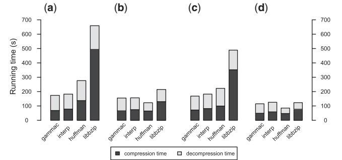
Fig. 7. Compression and decompression (including transformation) times averaged over three trials for SRR032209. Lossless transformation GapTranslating and no lossy transformation for (a) k=1 and (b) k=256 ; and with no lossless transformation and lossy transformation LogBinning at |\Sigma|=5 for (c) k=1 and (d) k=256 .
