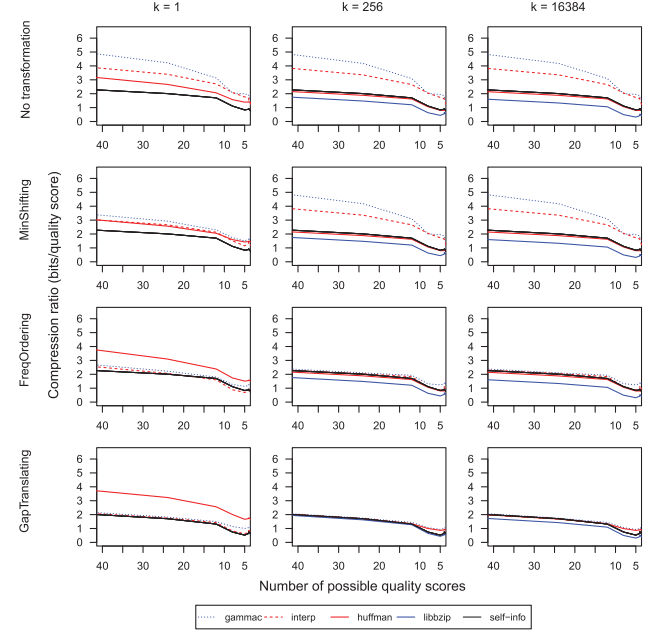
Fig. 6. Compression effectiveness achieved with LogBinning for SRR032209, with k and |\Sigma| varying on the horizontal, and lossless transformations varying on the vertical dimensions. Black lines represent the self-information, which is unaffected by block size.
