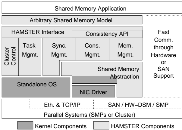
Figure 1. The HAMSTER Framework
