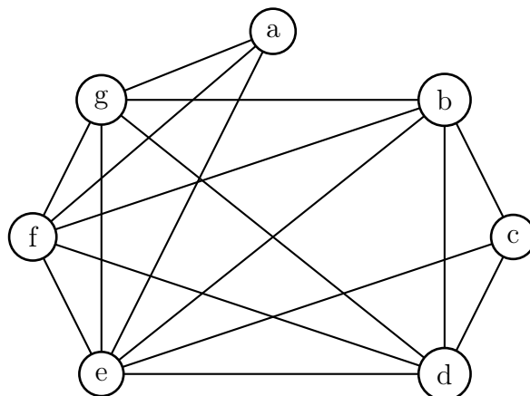
FIGURE 1 – Graphe G
