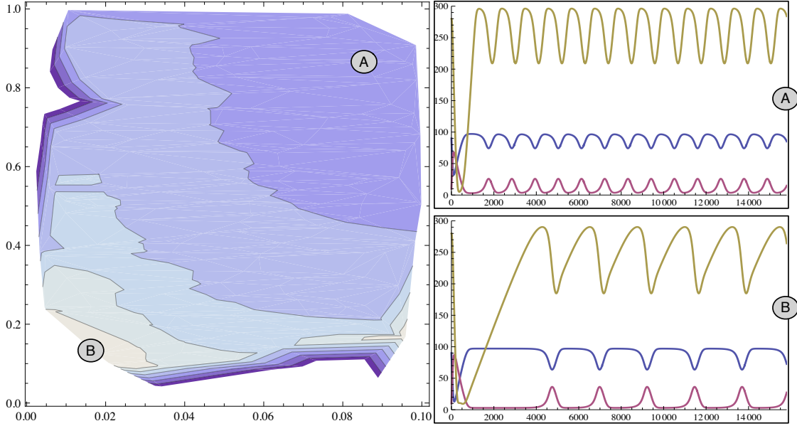
Figure 4.7: Oscillation period for the MAPK cascade model. Left: Contour plot representing the period of oscillations. The bottom axis (resp. left axis) represents values of the k_4 (resp. v_5 ) parameter. The contour plot was built with 500 simulations with random parameters. Regions with comparable periods are represented by a uniform region. Right: Two example trajectories exhibiting oscillations of extreme period A:1094 time units and B:2236 time units.
