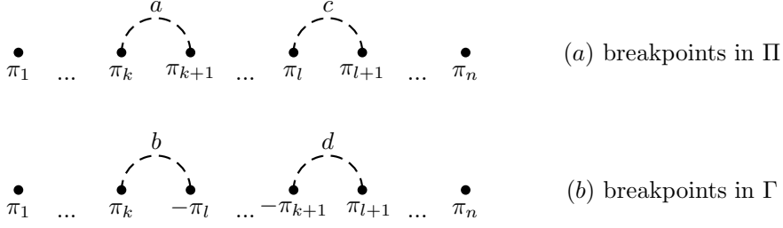
Figure 3.6: \Pi and \Gamma are identical up to a, c (or b, d ). This implies (a) the existence of 2 breakpoints a = \pi_k.\pi_{k+1} and c = \pi_l.\pi_{l+1} in \Pi , and (b) of 2 breakpoints b = \pi_k.-\pi_l and d = -\pi_{k+1}.\pi_{l+1} in \Gamma .
