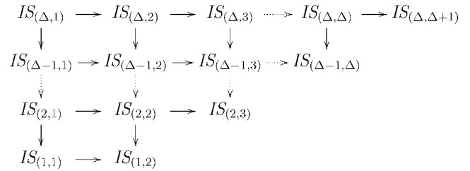
FIG. 2. Illustration of the time ordering of independent set construction.
