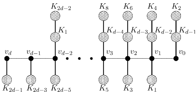
FIG. 1. A graph which requires \Omega(d) time to LF-color in the distributed model.
