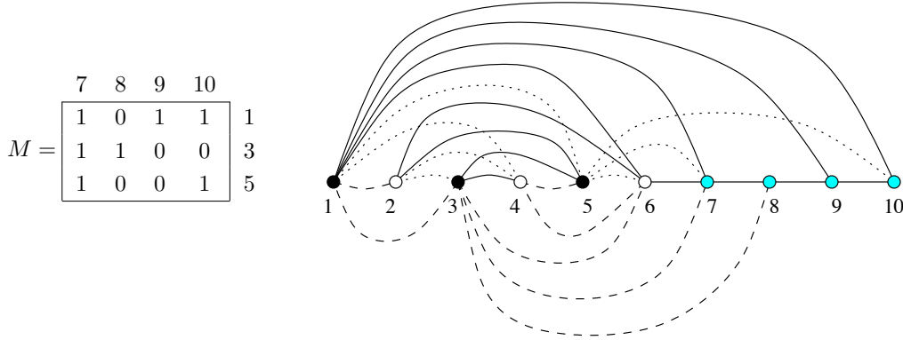
Fig. 2: Construction of an n -node graph of pagewidth k = 3 . The matrix M denotes adjacency between the nodes \{1, 3, 5\} and \{7, 8, 9, 10\} . Solid, dashed and dotted lines correspond respectively to page 1, 2 and 3.
