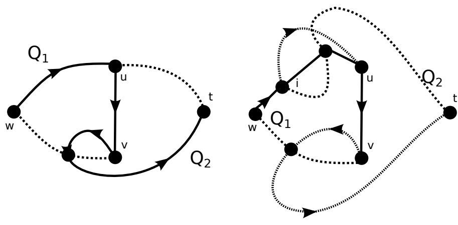
Figure 6: The two cases for Q_1 and Q_2 . The big dots represent the paths' unused portions.
