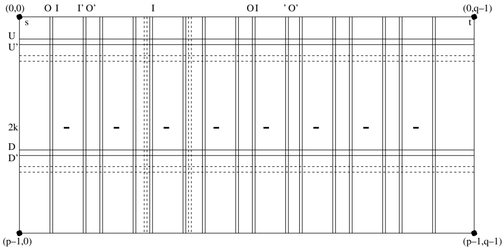
Fig. 1. Associated rows and columns.
