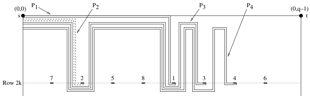
Fig. 2. The path P_s .
