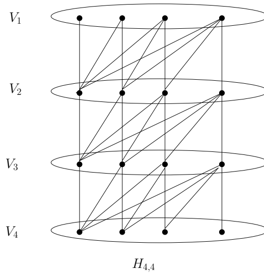
Fig. 2. The graph H_{4,4} . Each V_i , for 1 \leq i \leq 4 , induces a clique.
