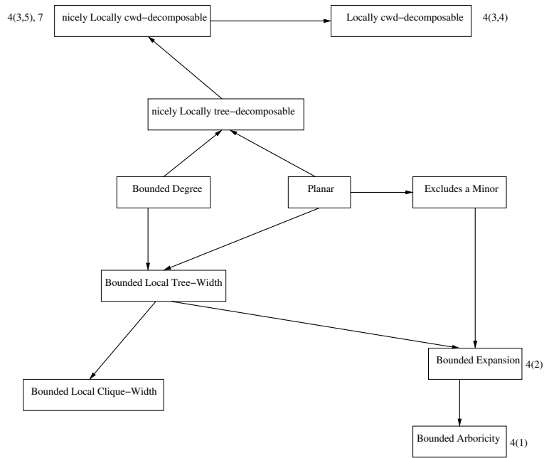
Fig. 1. Inclusion diagram indicating which results apply to which classes. An arrow means an inclusion of classes.
