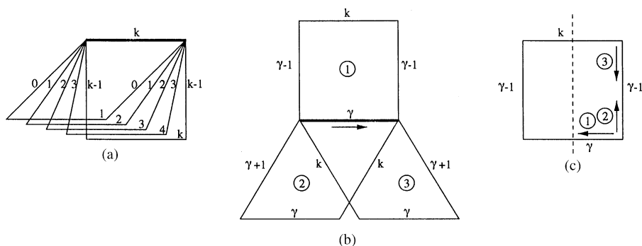
Fig. 3. The 4-cycles in a Knödel graph of order 2 \cdot 2^k .
