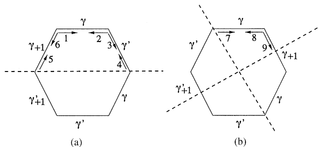
Fig. 4. (a) The six possible travels of the cycle of type (b) in Fig. 2(b). The three possible travels of the cycle of type (c) in Fig. 2.
