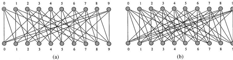
Fig. 1. A Knödel graph of 20 vertices (a), and a Fibonacci graph of 20 vertices (b).
