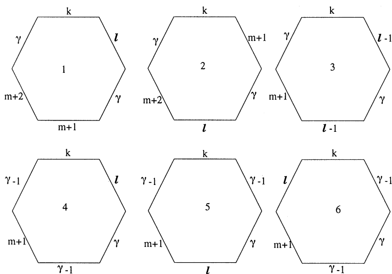
Fig. 8. Additional solutions provided by Eq. (3) with B_1(n') = 1 .
