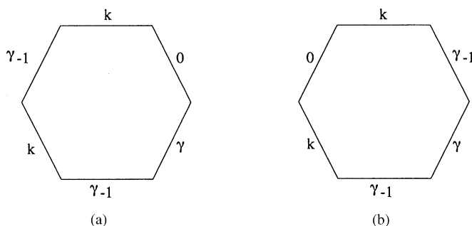
Fig. 9. Specific solutions for n = 2^{k+1} - 1 .
