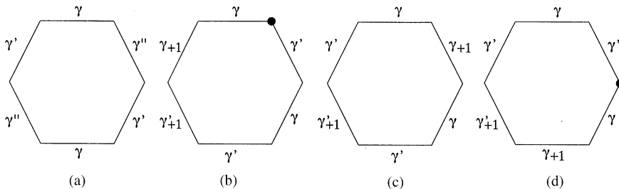
Fig. 2. The four types of solutions of Eq. (2) for \alpha = 0 .
