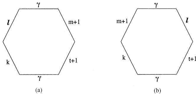
Fig. 7. Additional solutions provided by Eq. (3) if B_1(n') = 2 where \gamma \in \{0, \dots, k - 1\} \setminus \{\ell, m + 1, t + 1\} .
