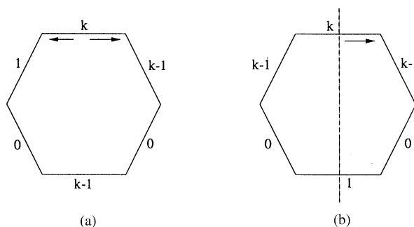
Fig. 5. The 6-cycles containing non-adjacent edges of dimensions 0, 0, and k .
