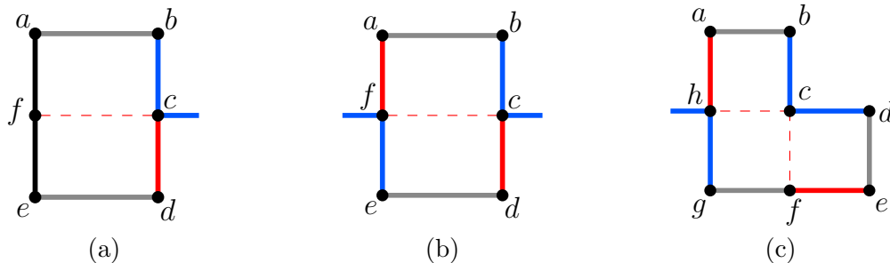
Figure 6: Illustration of Lemmas 4 and 5: (a) (c, f) is the missing edge of a 2-cell face and f is a boundary vertex, (b) (c, f) is the missing edge of a 2-cell face and none of c and f are boundary vertices, and (c) (c, h) is a missing edge of a 3-cell face.
