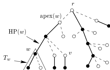
Fig. 1. Heavy nodes are black and light nodes are white. Heavy edges are solid and light edges are dashed. Heavy paths are subtrees composed of heavy edges only. In this example, \text{apex}(v) = v .
