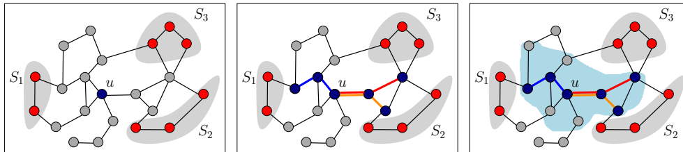
FIG. 4.1. An iteration of the algorithm. On the left, there are three supernodes S_1, S_2, S_3 neighboring the current component with u as a root. In the middle, we have a tree T_4 comprised of three shortest paths from u . On the right, the new supernode S_4 which is a 1-neighborhood of T_4 (observe that this neighborhood is taken in the connected component containing u ).
