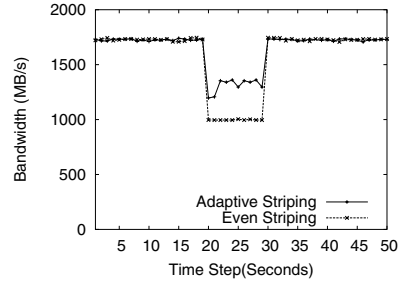
Figure 20. MPI Bandwidth with Adaptive Striping
