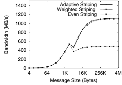
Figure 18. MPI Bandwidth with Adaptive Striping (UP mode)
