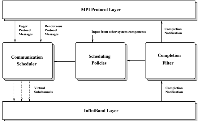
Figure 2. Basic Architecture of Multirail MPI Design
