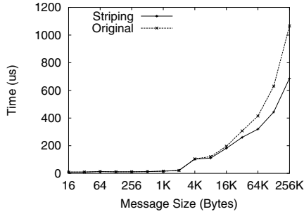
Figure 11. MPI.Bcast Latency (UP mode)
