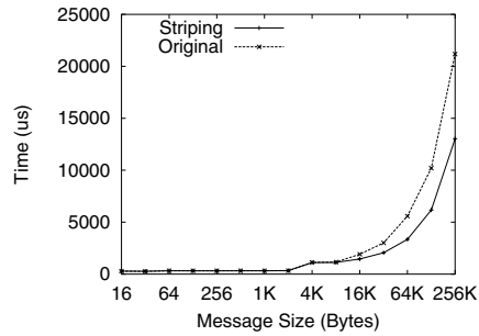
Figure 14. MPI.Alltoall Latency (SMP mode)
