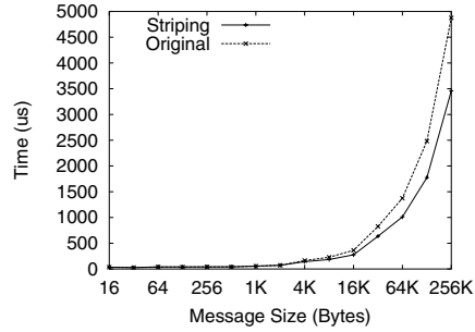
Figure 12. MPI.Alltoall Latency (UP mode)
