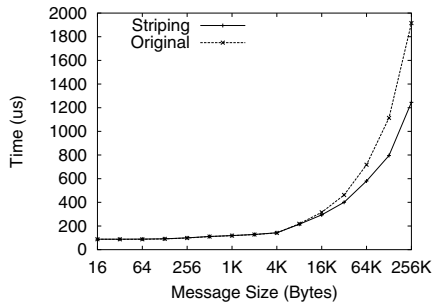
Figure 13. MPI.Bcast Latency (SMP mode)
