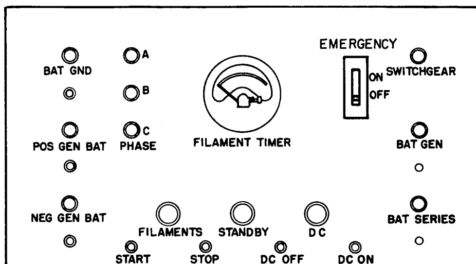
SWITCHGEAR PANEL - POWER SUPPLY
