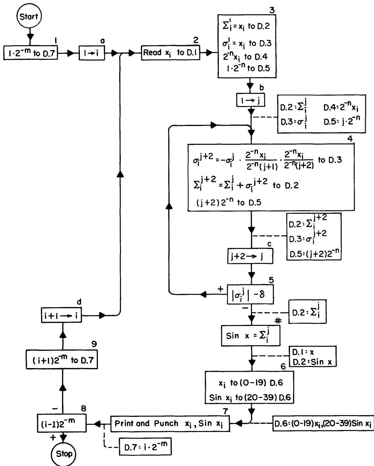
SINE by TAYLOR'S SERIES EXPANSION
