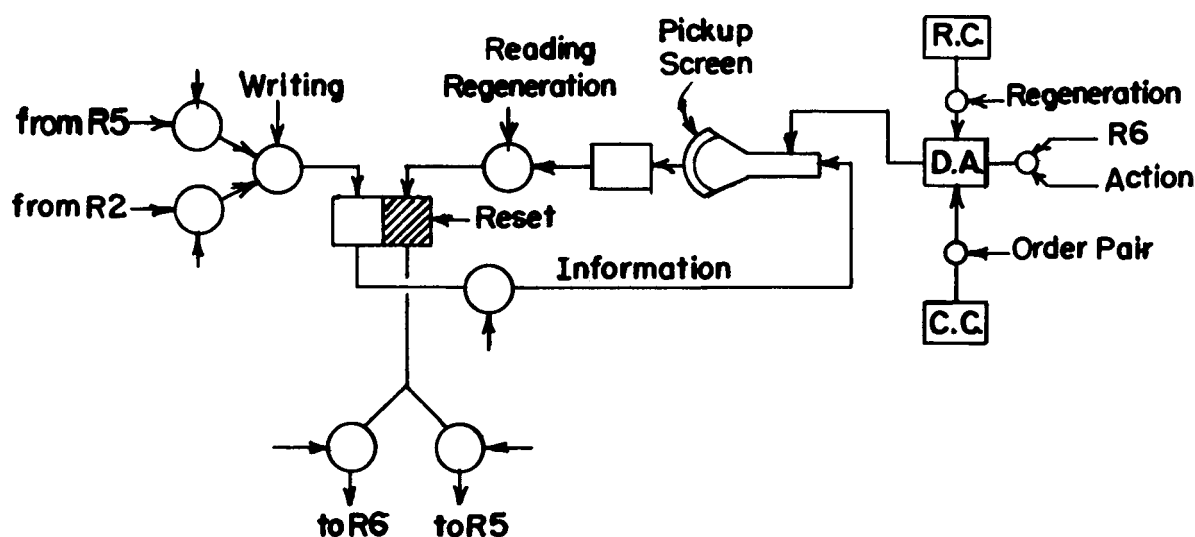
Fig. 5 Memory System. Abbreviations: D.A. deflection adder R.C. regeneration counter C.C. control counter
