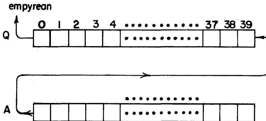
Fig. 2 Nature of left shift operation, showing interconnection of A and Q.
