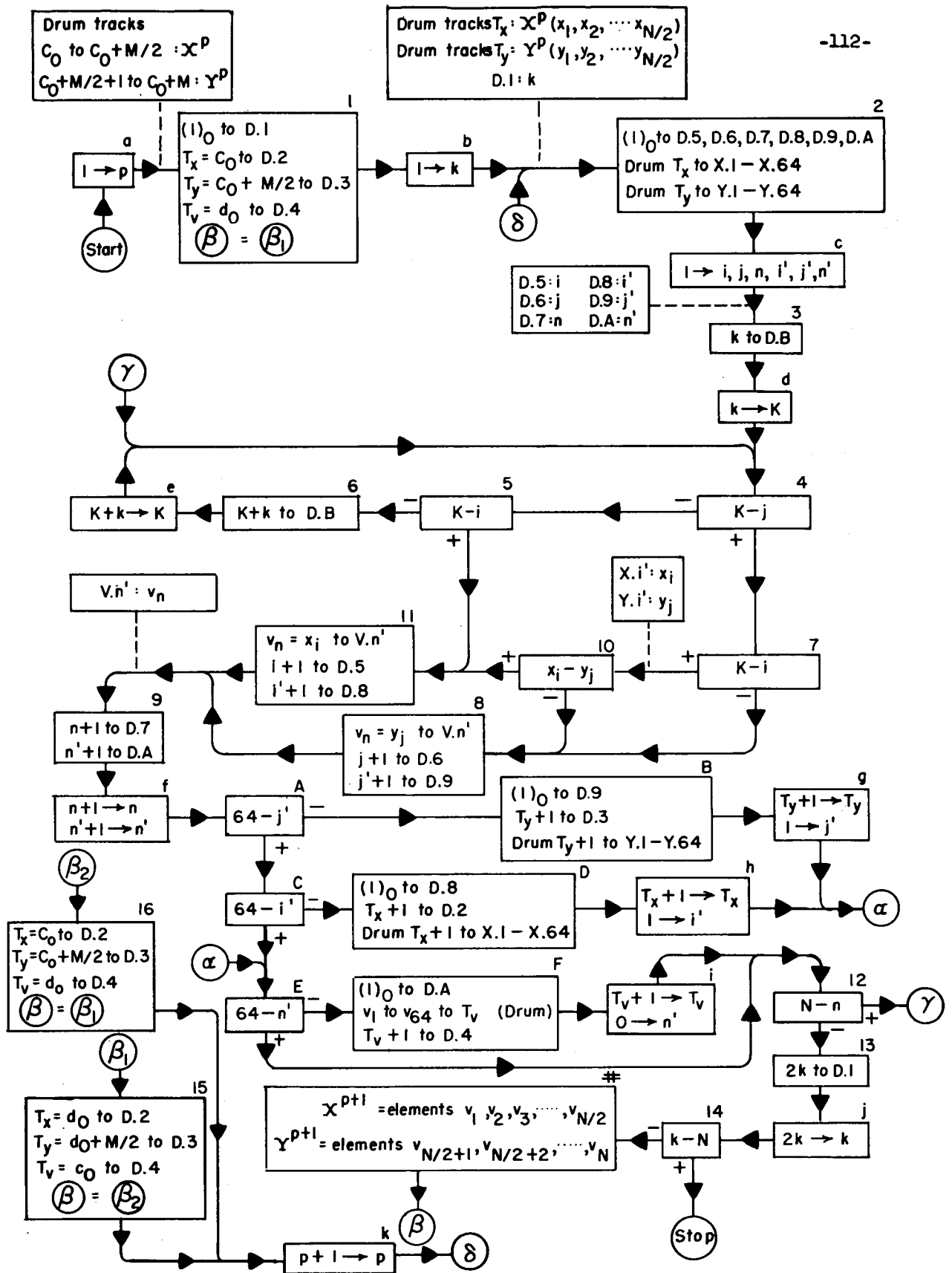
A SIMPLE SORTING PROCEDURE
