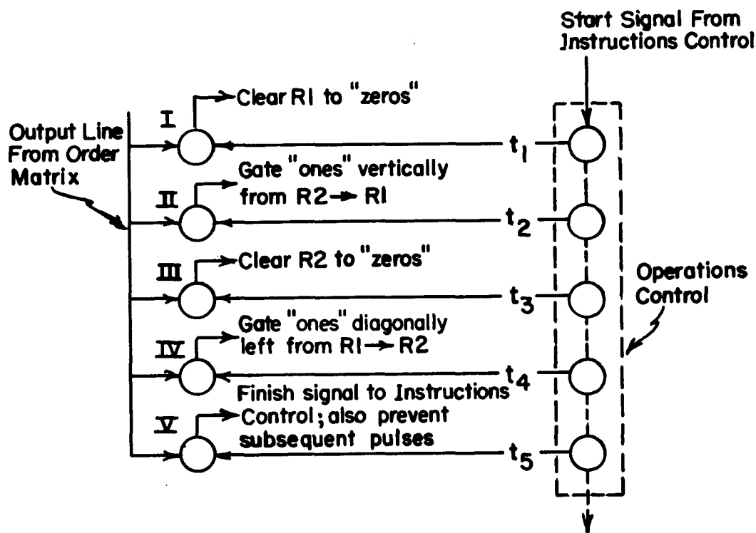
Fig. 9 Gate connections for a simplified order.
