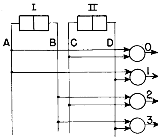
Fig. 8 A two stage order matrix.
