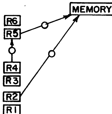
Fig. 7 Gate connections to the memory from the arithmetic unit.
