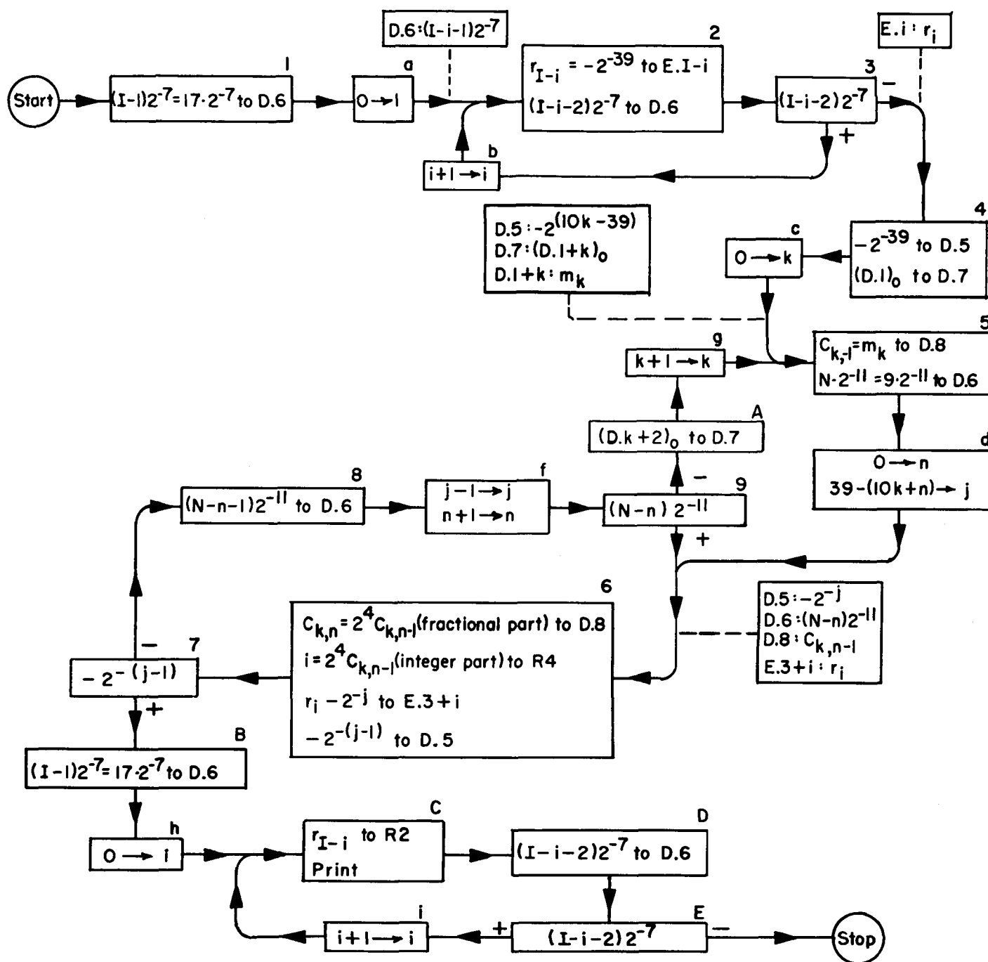
A SYNCHROPRINTER ROUTINE
