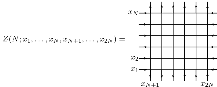
FIGURE 3. Partition function for ASM's of size N
